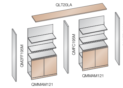
Mobile con fianchi finali e fianco centrale in melaminico Cupboard with melamine final and central side panels
