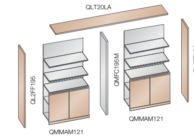
Mobile con fianchi finali in legno e fianco centrale in melaminico Cupboard with wooden final panels and melamine central side panel
