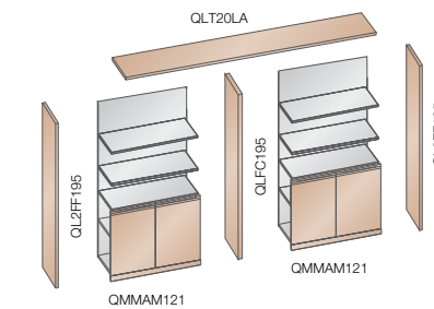
Mobile con fianchi finali e fianco centrale in legno Cupboard with wooden final and central side panels
